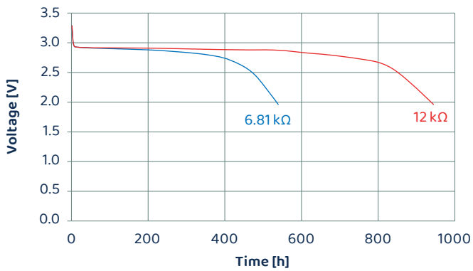
Discharge performance at 23 °C
