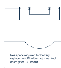
Layout top view
