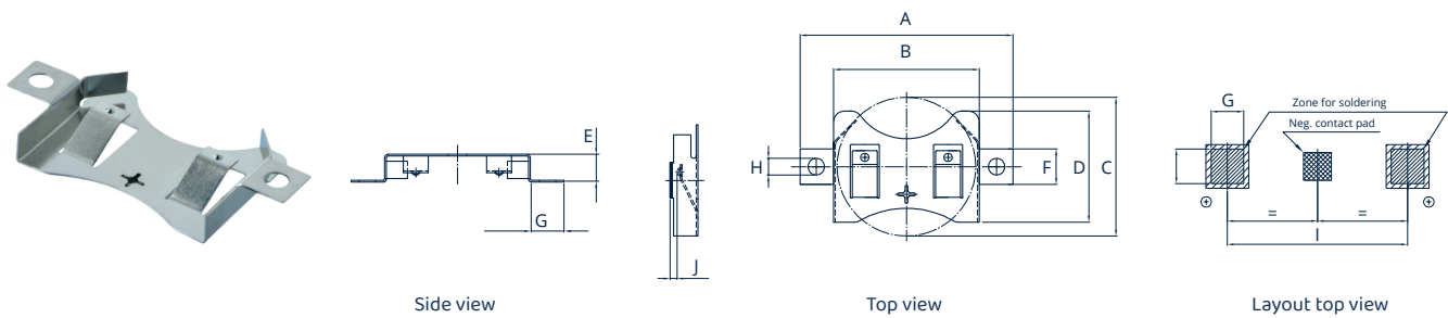
Maximum dimensions [mm]
