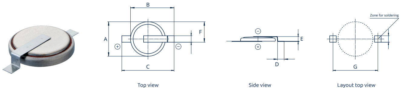
Dimensions [mm]
