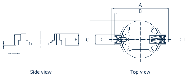
Dimensions [mm]
