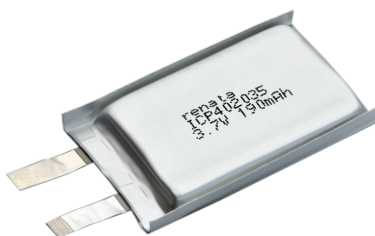
No safety circuit + Tab contact
