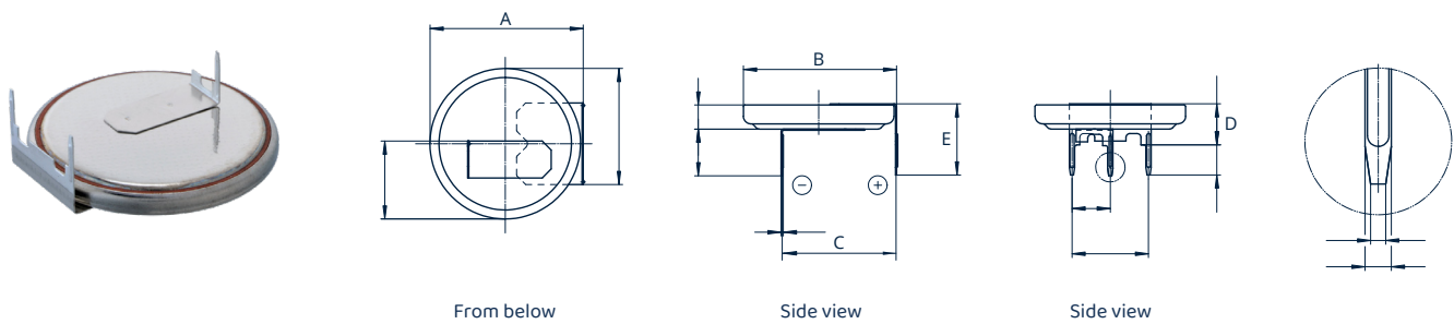
Dimensions [mm]
