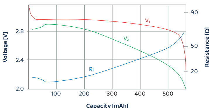
Figure: Pulse-current discharge characteristics 1 of the CR2450N cell. CR2450N Pulse intensity 10 mA, pulse width 50 ms, period 1 s. Cut-off voltage: 2.0 V
