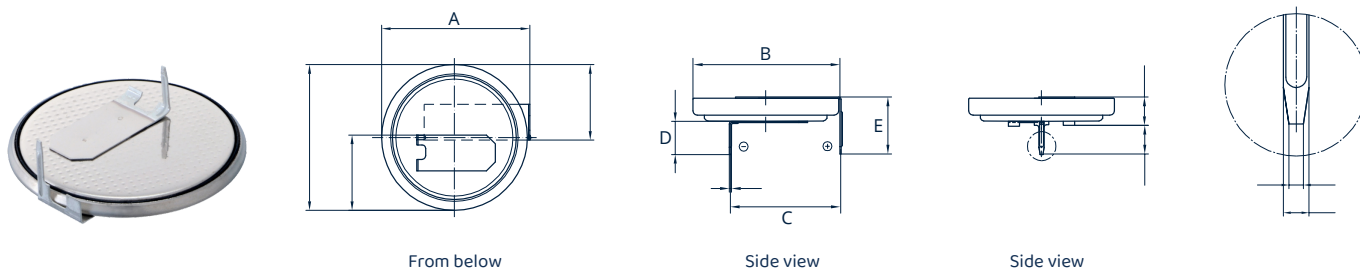
Dimensions [mm]
