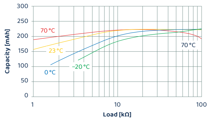
Cell capacity at various loads
