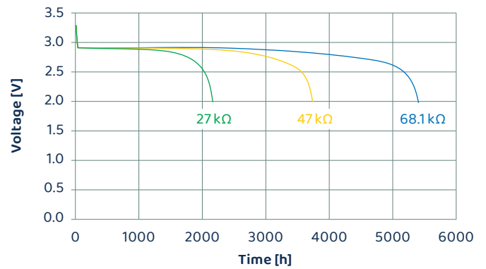
Discharge performance at 23 °C
