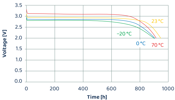
Temperature performance – Load 12 kΩ
