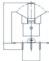
Front view from (+) pole side
