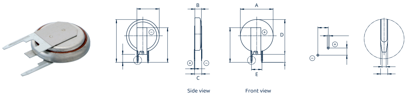
Dimensions [mm]
