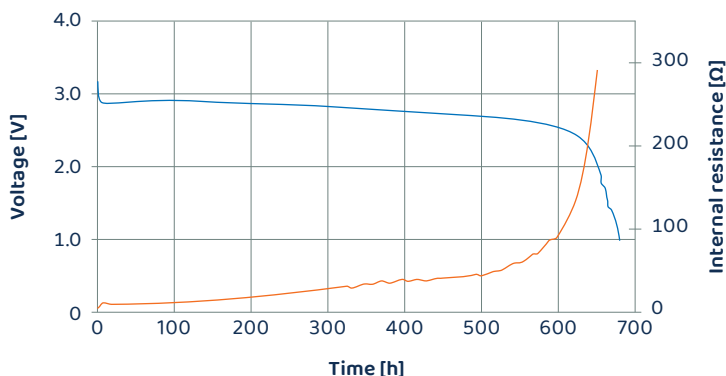
Figure: Characteristic curve of a CR2450N cell. Discharge load: R_1 = 3.32 \text{ k}\Omega . Measurement of internal resistance during discharge: by applying the load R_2 = 150 \Omega for 1 s, every 3 hrs.
